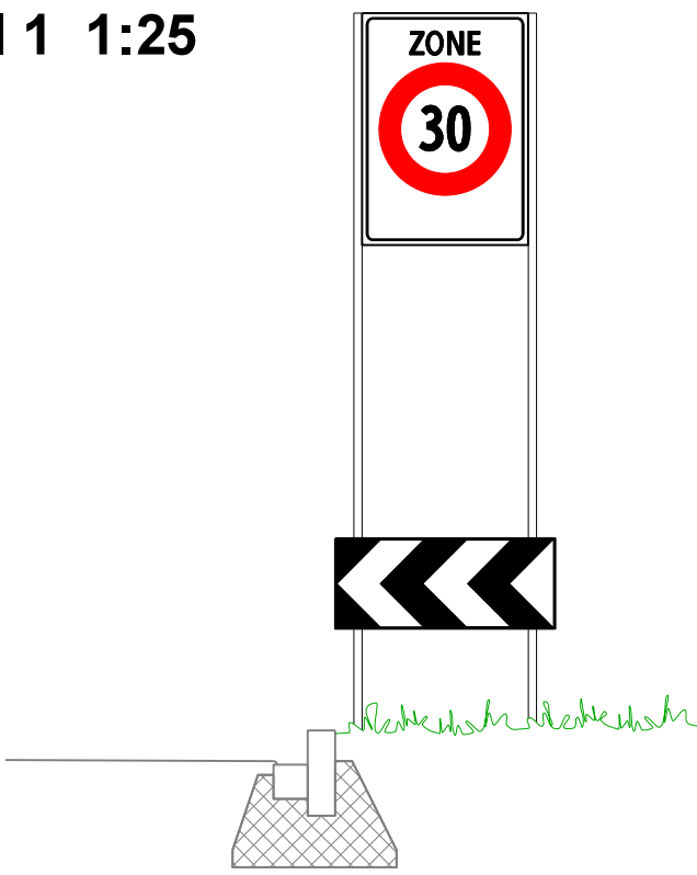
Detail 1 1:25
