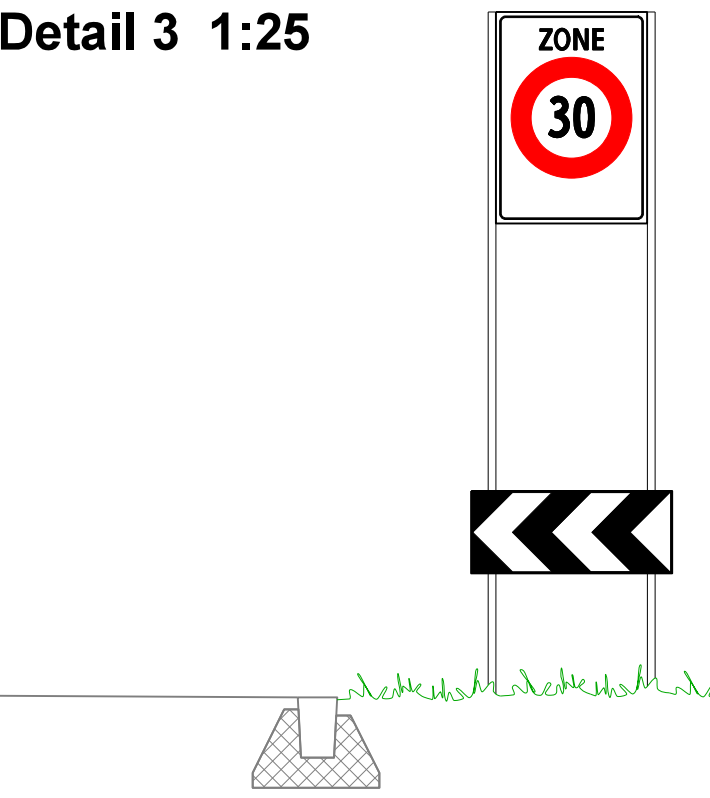
Detail 3 1:25
