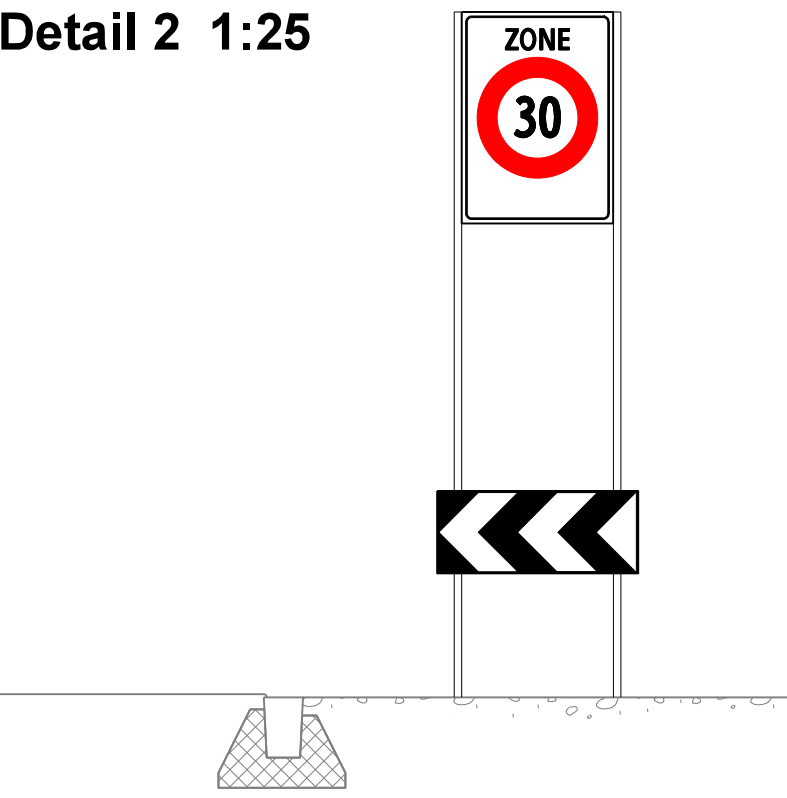
Detail 2 1:25
