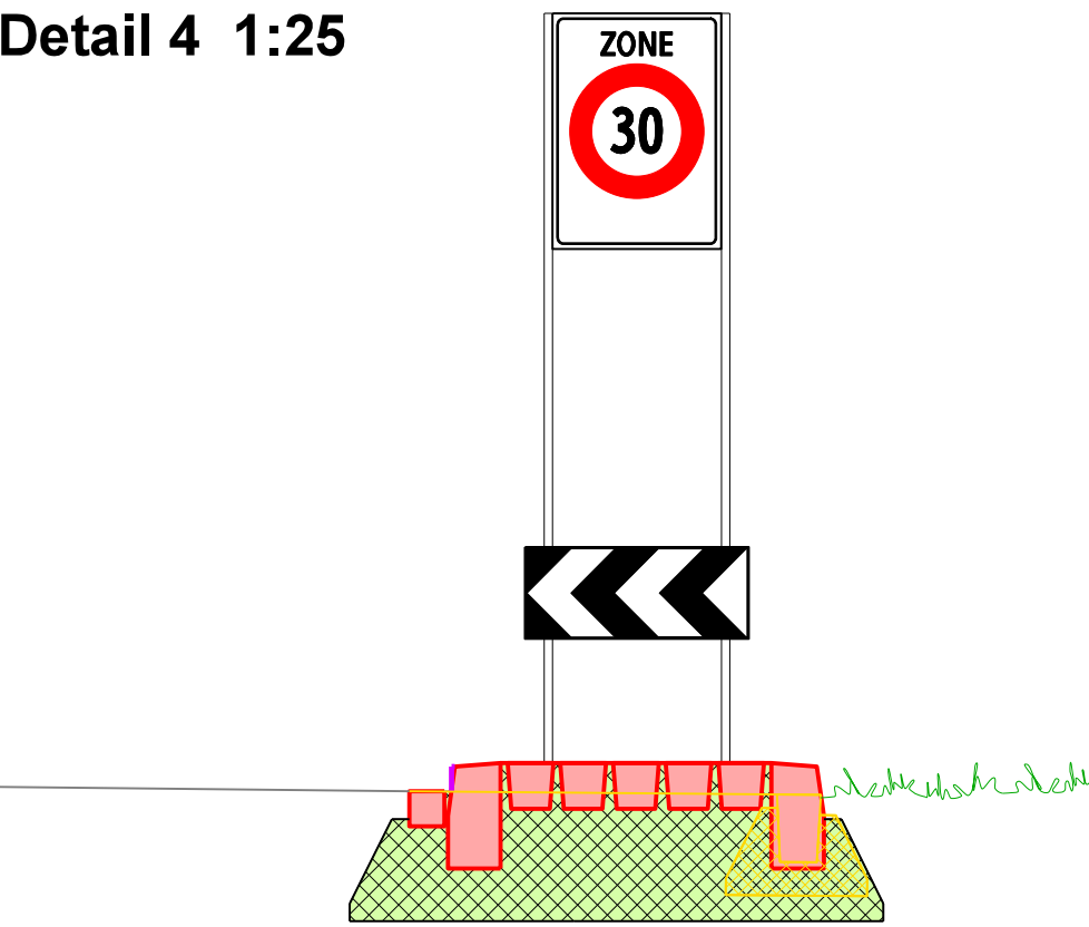
Detail 4 1:25
